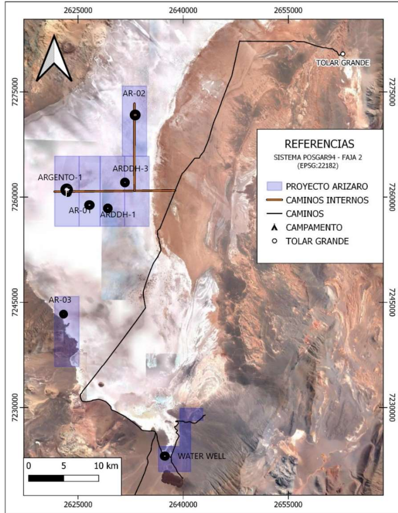
Figure #2 – Phase 2 Exploration Campaign - Proposed Well Locations, Arizaro, Argentina
